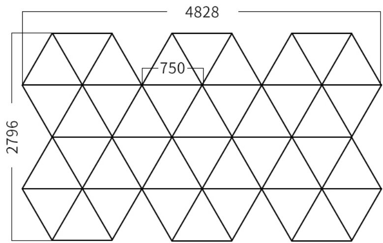
Hexagonal Grid Light-Link Superior Brightness, Versatile Use, Energy Efficiency Model: SGGF285 Specification: 6500K/2796*4828mm/AC110-240V/710W/110lm/w
